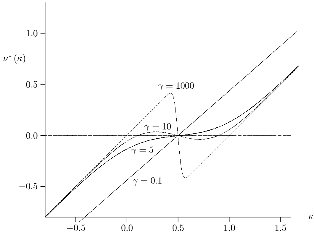
Figure 3.2: Function \nu^*(\kappa)
